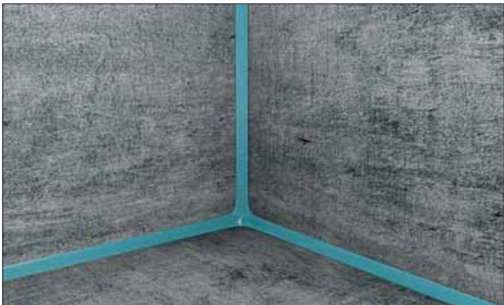
● Inside corner formed with silicone joint
